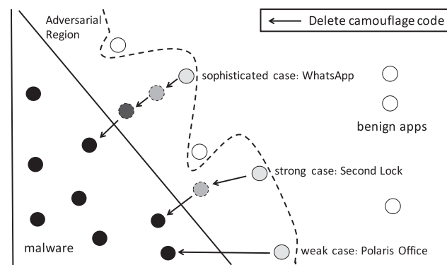
Fig. 3 – The process from benign to malicious: the black dots refer to malicious apps, the white dots refer to benign apps, and the gray dots are originally malware but misclassified as benign due to the camouflage code injected in the adversarial region. The gray dots turn darker with the deletion of camouflage code and finally turn all black, exposing its malicious nature. The arrows direct toward the transformation process.
