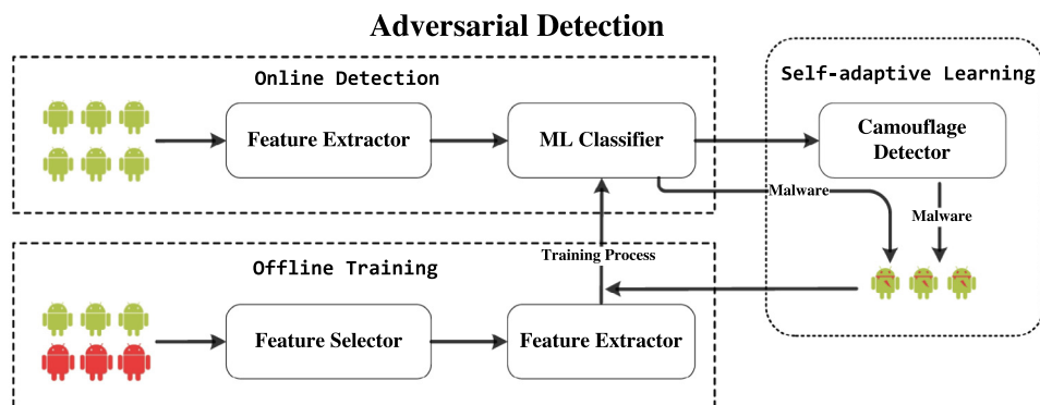
Fig. 6 – The KUAFUDET framework through adversarial detection.
